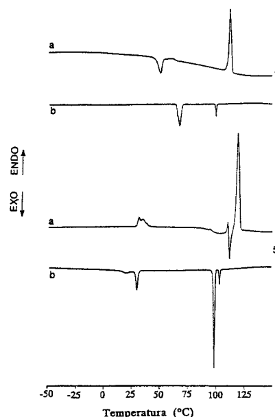
Slika 2: DSC-krivulje C5- in C6-diolov. (a) drugo segrevanje, (b) drugo ohlajanje, (n) število metilenskih skupin v oligometilenski verigi Figure 2: DSC traces of the C5- and C6-diols. (a) the second heating, (b) the second cooling, (n) the number of methylene units in alkyl chain
