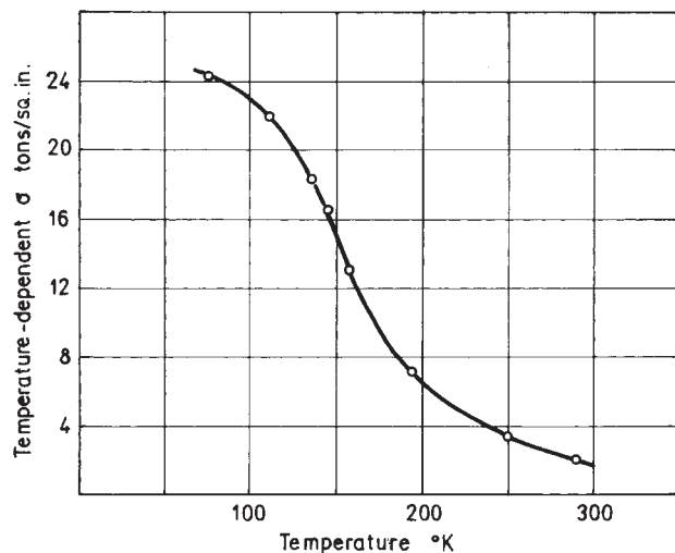
Figure 9: Effect of temperature on the temperature dependent component of the dislocation gliding friction force. From ref. 29
