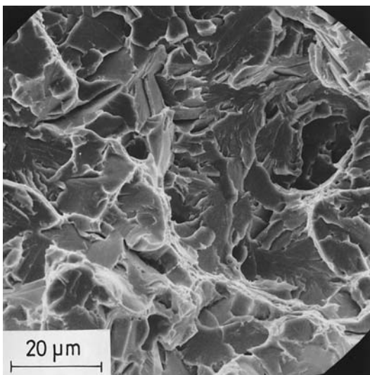
Figure 7: Lower shelf fracture surface of a CVN specimen of steel 1
