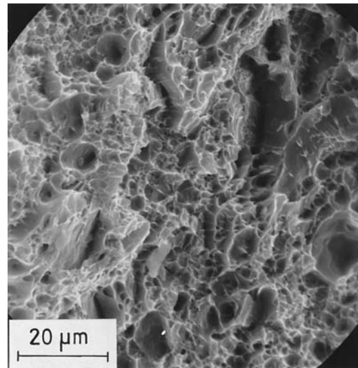
Figure 5: Dimpled ductile fracture surface of an unnotched tensile specimen of steel 1 broken at NDT (-125°C)
