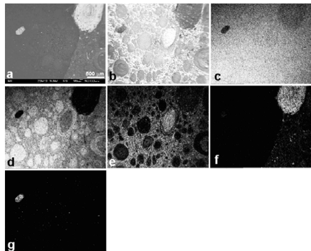
Figure 5: EDS X-ray mapping of Muljava 3 grinded sample (a) backscattered-electron image, (b) secondary-electron image and corresponding X-ray images (c) O K_{\alpha 1} (d) Al K_{\alpha 1} (e) Si K_{\alpha 1} (f) Fe K_{\alpha 1} (g) Ti K_{\alpha 1}
