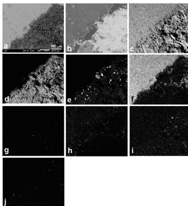
Figure 7: EDS X-ray mapping of Muljava 3 grinded sample (a) backscattered-electron image, (b) secondary-electron image and corresponding X-ray images, (c) O K \alpha 1 (d) Al K \alpha 1 (e) Si K \alpha 1 (f) Fe K \alpha 1 (g) Ti K \alpha 1 (h) Mn K \alpha 1 (i) K K \alpha 1 (j) Ca K \alpha 1
