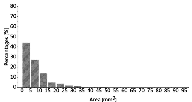
Figure 7: Histogram of the grain average area for the sample milled for 50 h and annealed
