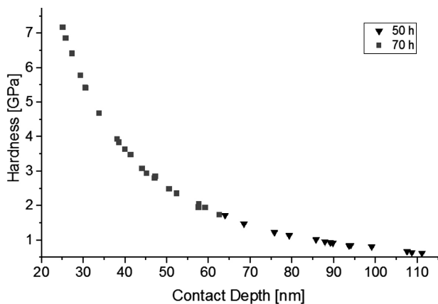
Figure 14: Diagram of hardness to contact depth for both samples, after 50 h and 70 h of milling
