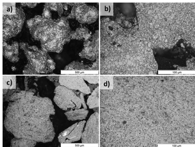
Figure 5: a), b) Optical micrographs of Ti-26Nb (a%) at different magnifications, produced in different milling times – 50 h and c), d) 70 h and annealing
