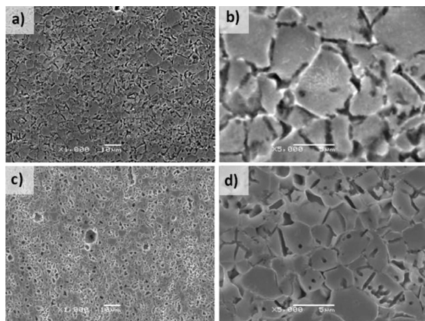
Figure 6: a), b) SEM micrographs of Ti-26Nb (a%) after different milling times – 50 h and c), d) 70 h and annealing
