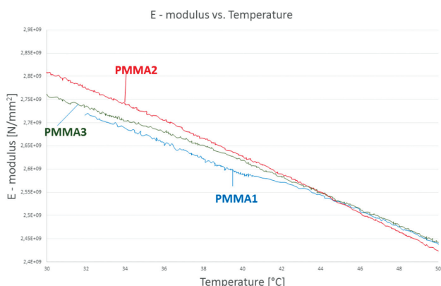
Figure 4: DMA results- diagram E – modulus ( N/mm^2 ) – T ( ^{\circ}C ) for all samples
