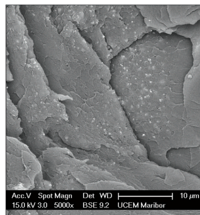
Figure 8: Micrographs of characteristic surface fracture in PMMA2
