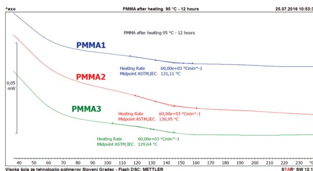
Figure 6: Results of flash DSC analysis for all samples, heating 1.000^{\circ}C/s (diagram heat flow ( mW ) – T ( ^{\circ}C ))
